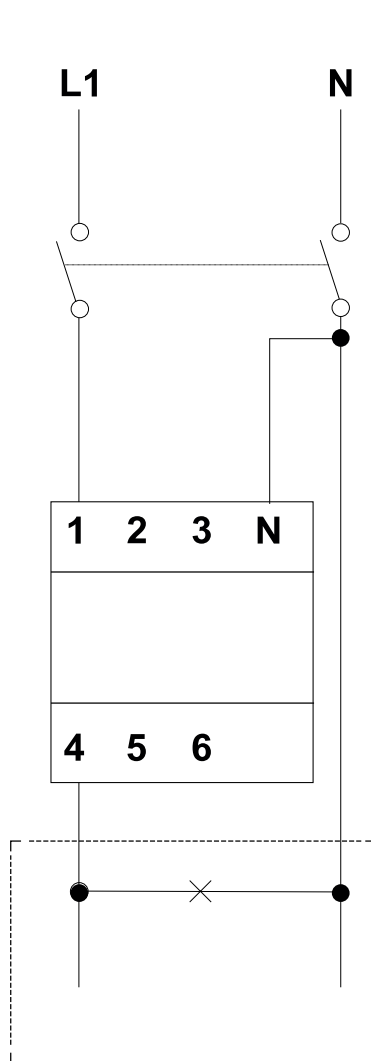
Single-phase system
