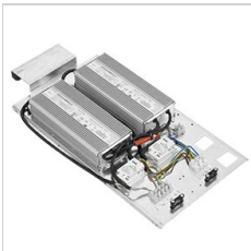
3104830 Drivers unit 470 W - 1.1A - 2CH - DALI - 220-240 V 50/60 Hz
