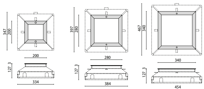
STEEL SQUARE 20
